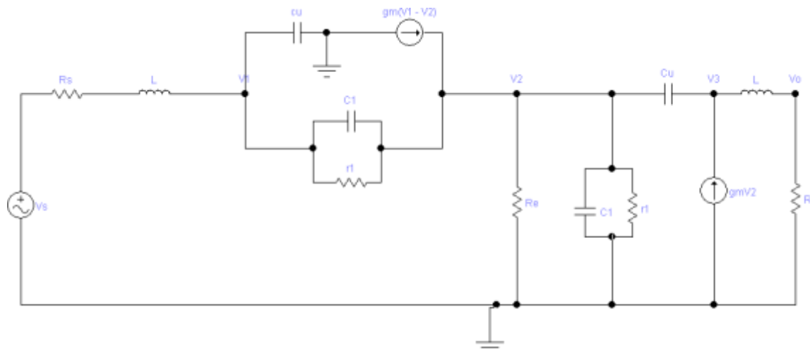
Figure 3: Ac Equivalent Circuit for the Proposed Distributed Amplifier
