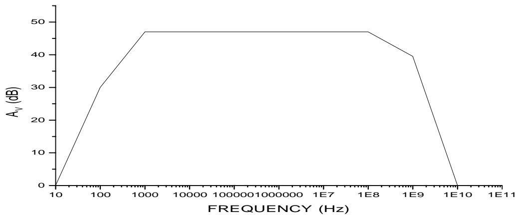
Figure 4: Frequency Response of the Distributed Amplifier (Simulation)
