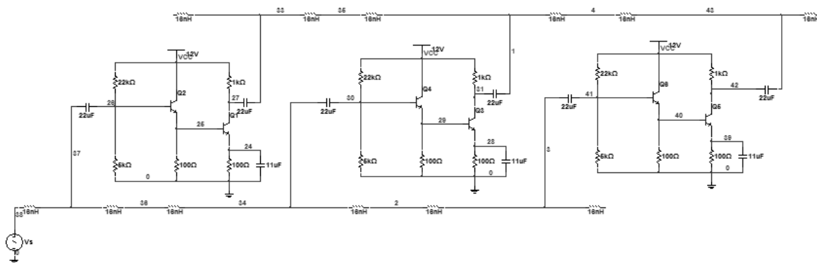
Figure 2: Schematic diagram of the distributed amplifier.
