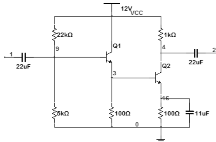
Figure 1: Schematic diagram of the conventional Darlington pair amplifier
