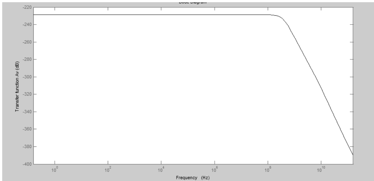
Figure 5: Frequency Response of the Distributed Amplifier (Theoretical)
